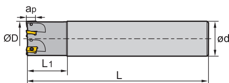
Straight shank
